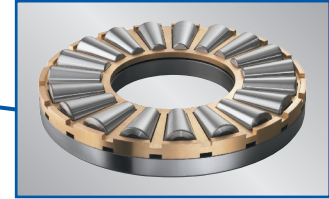
Heavy Duty Tapered Roller Thrust Bearings for Top Drives
